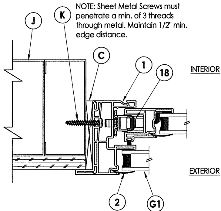
4 HORIZONTAL CROSS SECTION Shown w/ Steel Stud Framing Option
