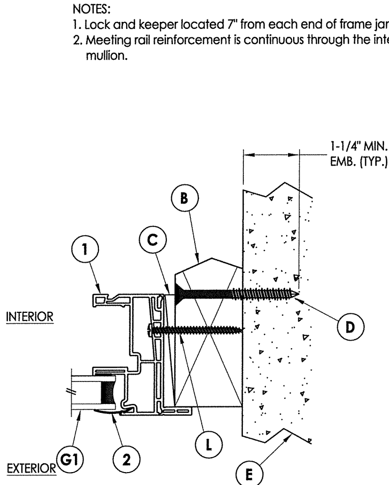
3 HORIZONTAL CROSS SECTION 2X Buck Masonry Construction
