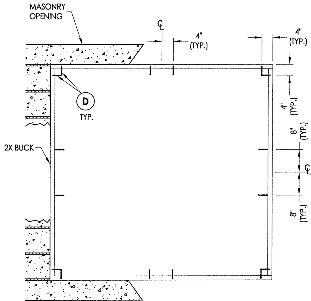
BUCK ANCHORING
