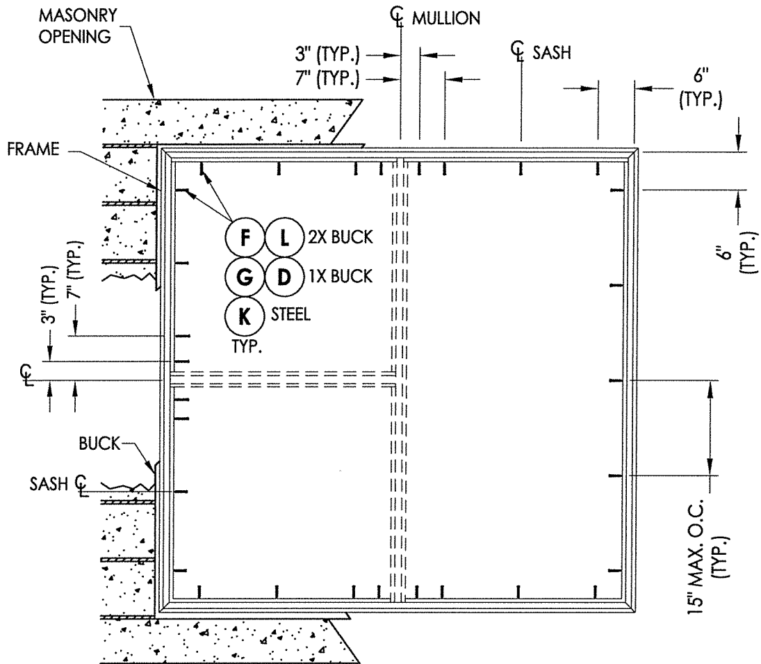
FRAME ANCHORING
