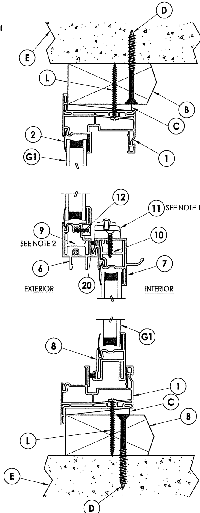
2 VERTICAL CROSS SECTION 2X Buck Masonry Construction
